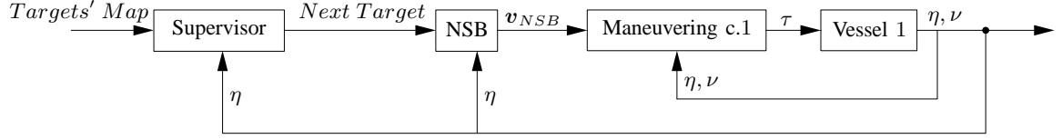
Fig. 1. Sketch of the guidance system control schema
