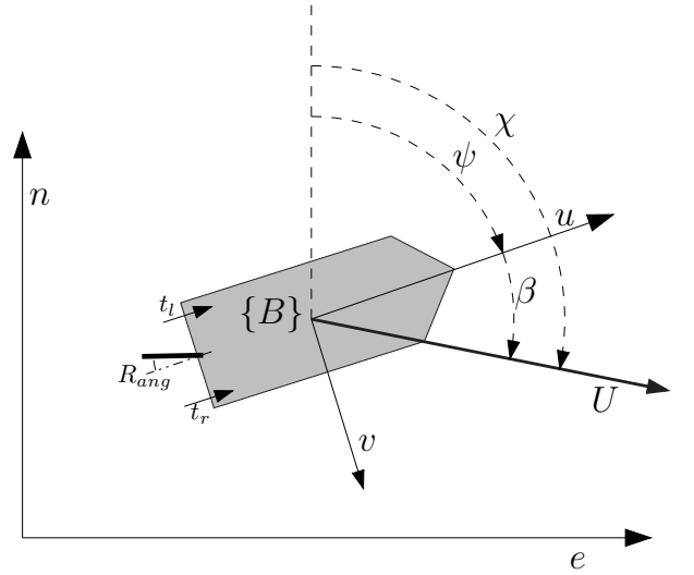
Fig. 3. Motion reference model of the surface vessel
