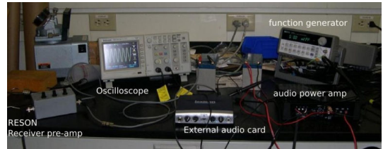
Fig. 3. The underwater acoustic communication testbed.
