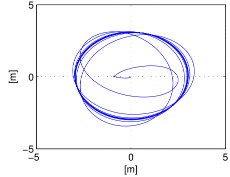
Fig. 12. Plot of the vessel path during a 1000s mission with a communication delay of 3s.
