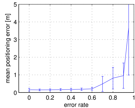
Fig. 9. Mean value and standard deviation of the positioning error for different error rate values with sample time t = .1s
