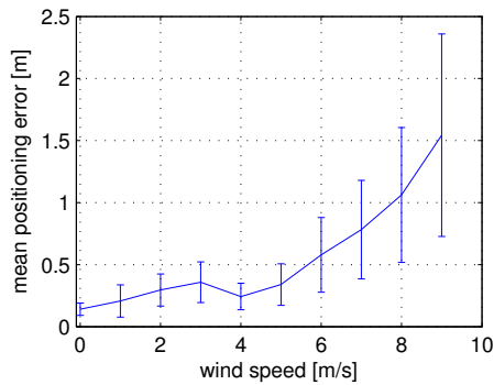
Fig. 15. Mean value of the positioning error for different values of the wind speed.
