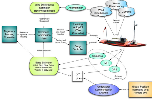
Fig. 8. Position control system with global positioning received from the onboard GPS or from a remote unit.
