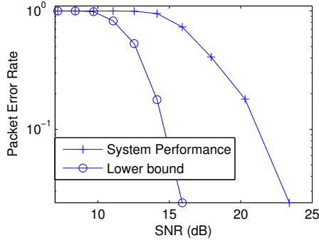
Fig. 6. Packet error rate vs. SNR.
