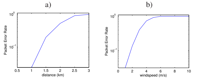
Fig. 7. a) Packet error rate vs. distance; b) Packet error rate vs. windspeed
