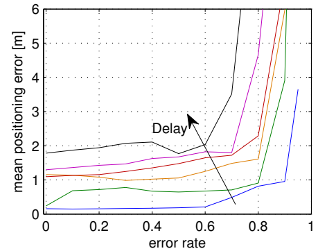
Fig. 13. Mean value of the positioning error for different error rate values for delay values of 0s, .3s, .6s, .9s, 1.2s, 2s
