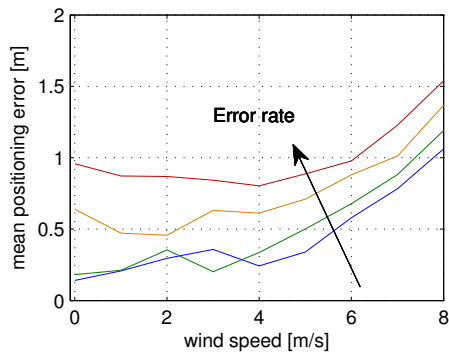
Fig. 16. Mean value of the positioning errors for different values of the wind speed with different error rate values (0, .5, .7, .8).
