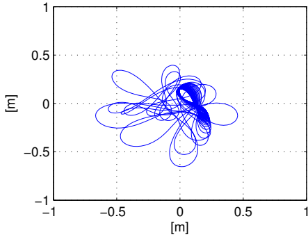
Fig. 11. Plot of the vessel path during a 1000s mission with a communication delay of 0s.
