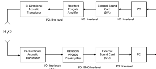
Fig. 4. Block diagram of a single link transmission in the underwater acoustic communication testbed.
