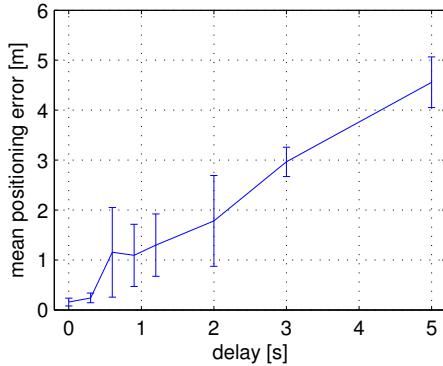
Fig. 10. Mean values and standard deviations of the positioning error for different delay values.
