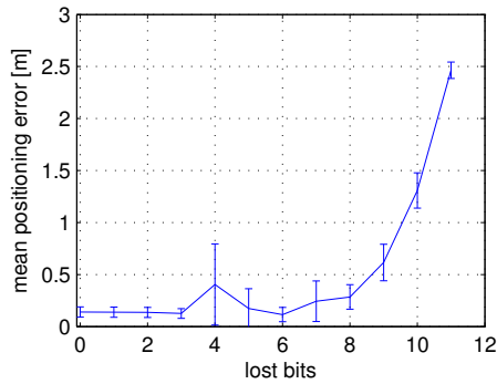
Fig. 14. Mean value of the positioning error for values of bit lost.
