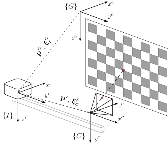
Figure 1: Global \{G\} , IMU \{I\} , and camera \{C\} reference frames, for target-based calibration. The transform from the IMU frame to the global frame is defined by the (\mathbf{p}^G, \boldsymbol{\xi}_I^G) translation and rotation pair. The transform from the camera frame to the IMU frame is defined by the (\mathbf{p}^I, \boldsymbol{\xi}_C^I) translation and rotation pair. A version of this figure appeared previously in [1].
