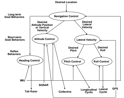
Fig. 2. Behavior-Based Controller
