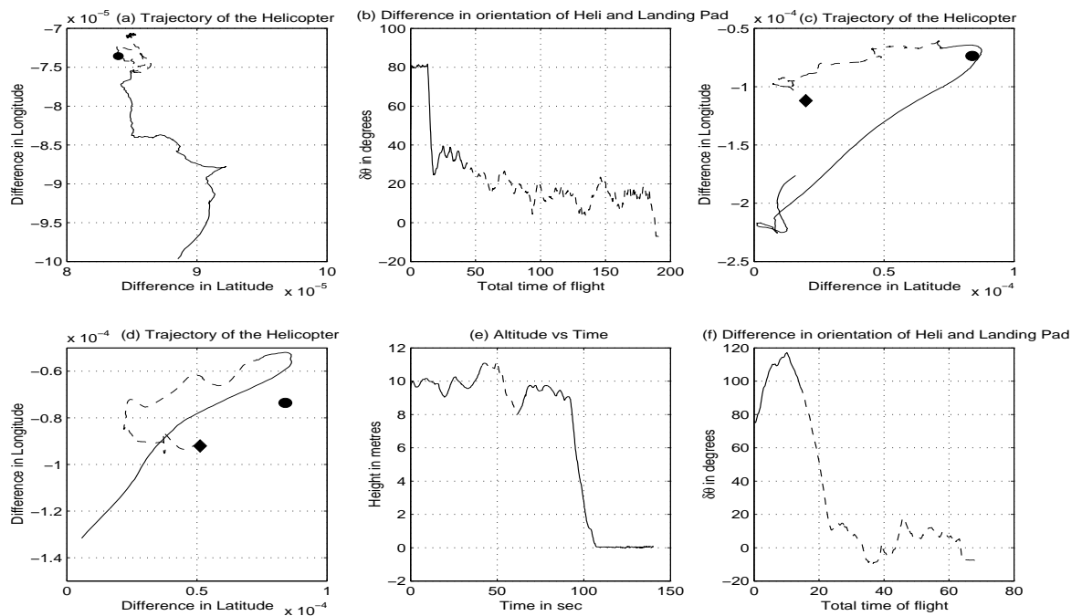
Fig. 3. Vision algorithm in conjunction with the landing controller (in the figure the circle represents the initial position of the helipad and the diamond represents the final position. The x - y axis of the graphs show the distance traversed by the helicopter from its initial location to the final location as a function of latitude and longitude)
