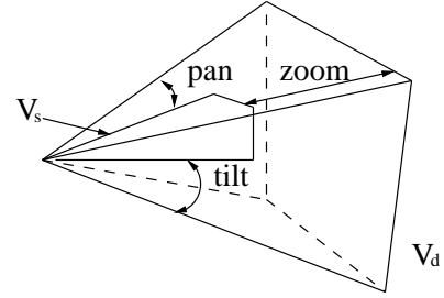
Figure 2. Model for detection volume and sensing volume.
