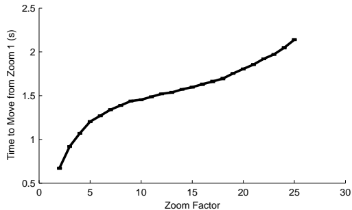
Figure 3. The time to actuate from the widest angle to various zoom factors for the camera used in our prototype.
