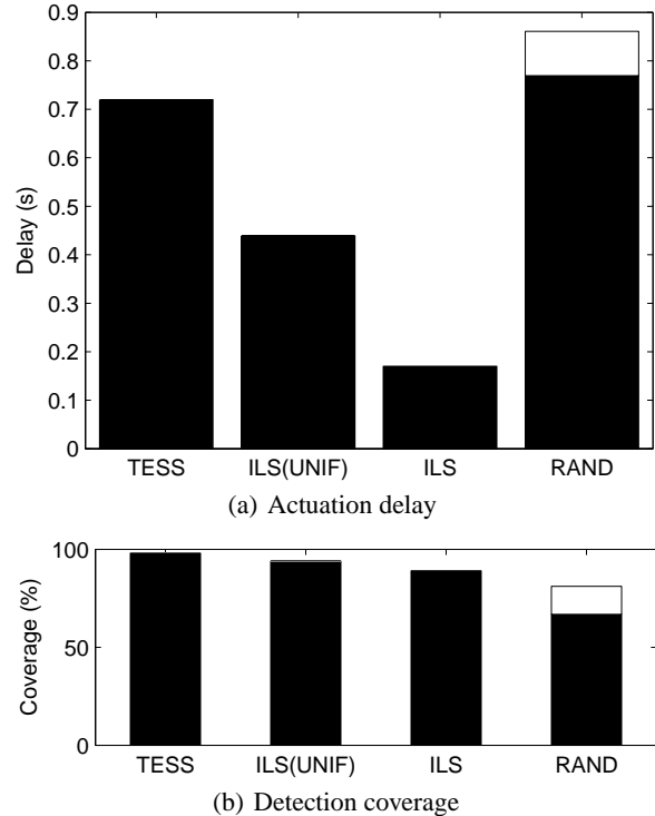
Figure 12. Performance of different network configurations, when optimization is weighted for actuation delay.
