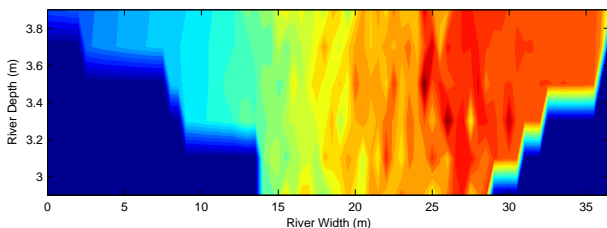
Figure 9. Nitrate concentration (mg/l) across the cross-section of a river.
