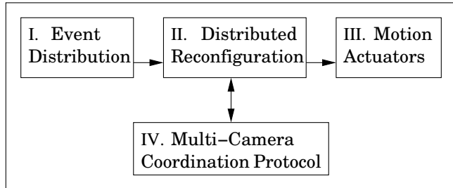
Figure 5. System software architecture.
