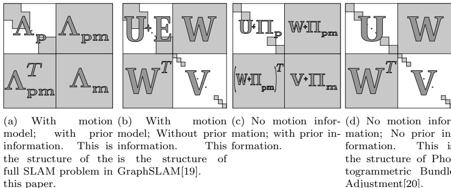
Figure 3: The pattern of the system matrix in the SLAM problem depends on information contributed (or not) from the dynamical process model and any prior information. With no process model information and no prior information the problem is equivalent to Photogrammetric Bundle Adjustment (the structure of this problem is visible on the right). Including a process model makes the upper left m \times m “process block” tridiagonal. Including a prior can potentially cause complete fill-in of the lower right n \times n “map-block”.
