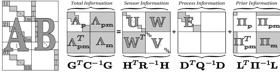
Figure 1: Basic structure of the sensor model Jacobian, \mathbf{H} .
