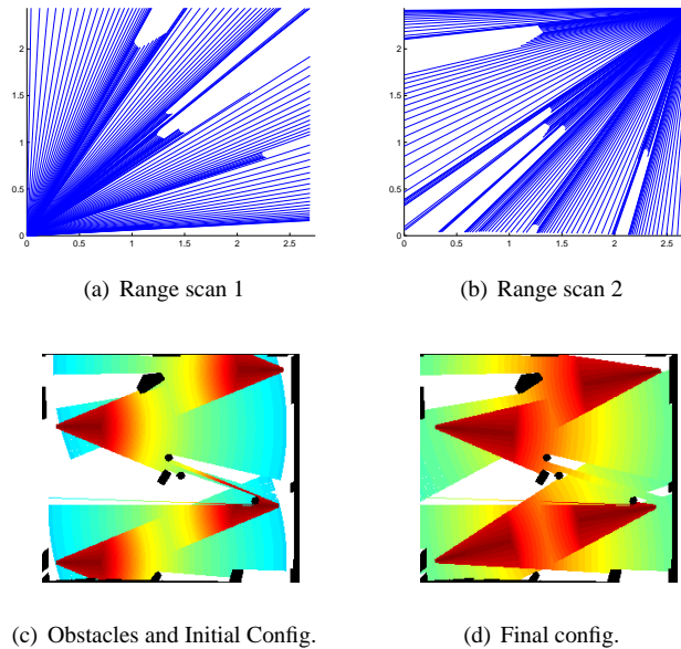
Fig. 12. ILS Optimization. The shaded sectors represent camera coverage, and the shade at a location corresponds to the spatial resolution achieved by the best camera for that location. (a) Range scan from laser in bottom left corner (b) range scan from laser in top right corner, (c) map of obstacles in the medium and the initial network configuration, (d) optimized configuration found by ILS - it changes both the pan and zoom settings of the cameras to increase sensing performance characterized by time required for recognition.
