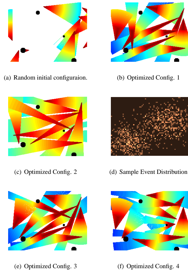
Fig. 9. ILS Optimization (a) random initial network configuration (b) optimized configuration with w = 0.1 , showing significantly improved coverage than (a), (c) optimized coverage using w = 0.9 , showing the different stable state than (b), (d) a sample event distribution, where brighter areas show higher event density (e) optimized configuration after learning the event distribution, and (f) optimized configuration with \alpha set to a high value.
