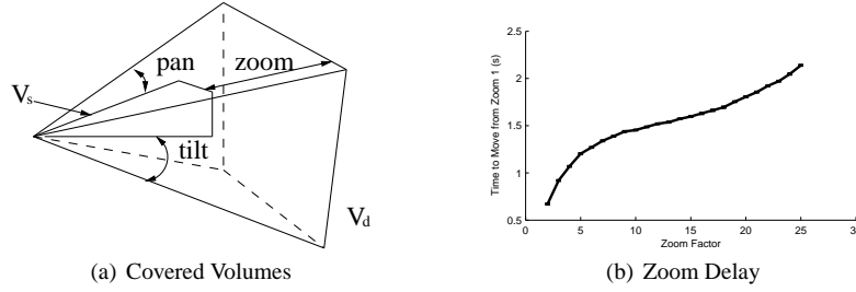
Fig. 4. (a) Covered volumes for detection and sensing phases, with the pan, tilt, and zoom required to provide sensing resolution within the detection volume. (b) The time to change zoom measured as a function of the zoom step. The communication delay in sending the zoom command was separately characterized and has been subtracted from the motion time.
