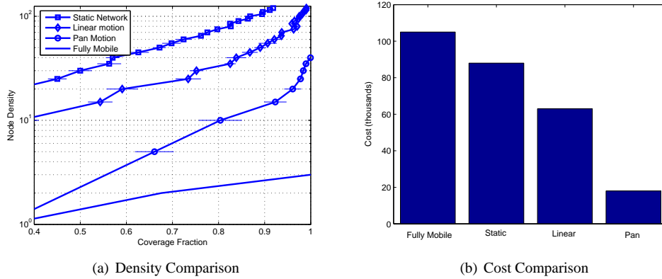
Fig. 6. Alternative deployments: (a) Coverage fraction with and without actuation at different deployment densities. Node density is the number of nodes in a 20m \times 20m square region, where each sensor covers a sector of 45^\circ with radius R_s = 7.3m . The error bars show the standard deviation across 10 random topologies simulated. (b) Converting the node density to total network cost, at 90% coverage point.
