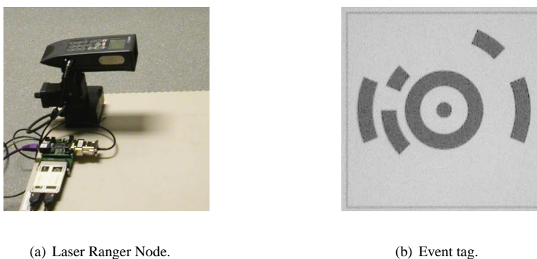
Fig. 3. System design (a) our prototype laser ranger node with pan and tilt capability, used to map the obstacles in the sensing medium, and (b) a sample tag, used as an event to be detected and recognized in our test-bed.
