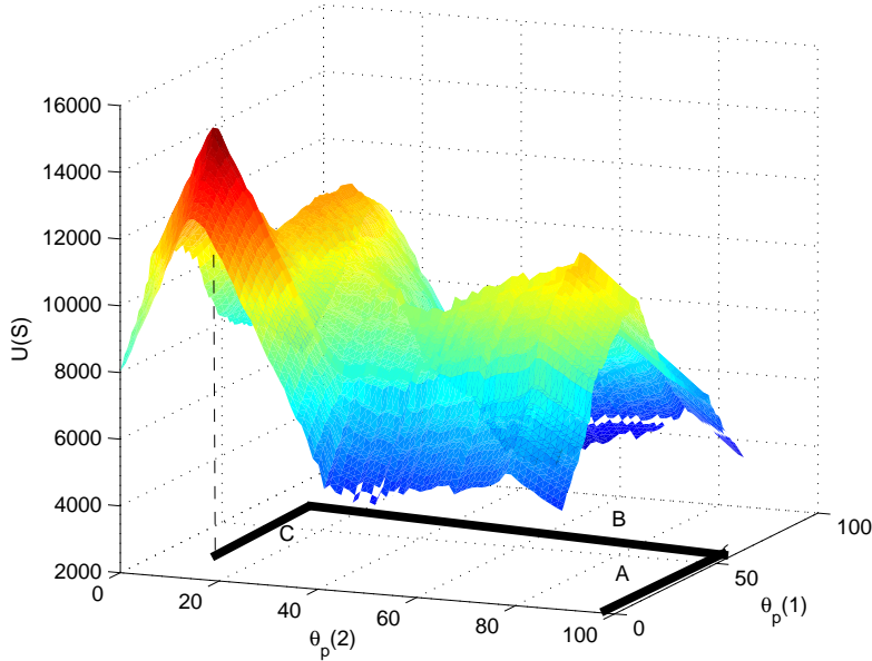
Fig. 7. Utility function for various possible pan pose combinations. The \theta_p values are in degrees, measured counter-clockwise from initial camera pose. The utility function has multiple local maxima, even for this simple scenario.
