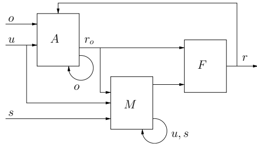
Fig. 2. Block-diagram of the fine-scale localization algorithm. The inputs are odometry data o (latitude, longitude and heading); IMU data u (roll and pitch) and laser scan data s (a set of range and bearing pairs). The output is the updated robot pose estimate r (latitude, longitude, altitude, and roll, pitch, heading). The first block A generates an updated pose estimate r_o based on the previous pose estimate r and the change in odometric pose; the second block M computes a corrected pose estimate r_s by comparing successive laser scans; the final filter block F combines these two estimates to produce the updated pose estimate r .
