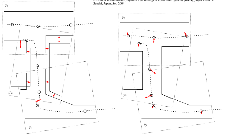
Fig. 6. Feature-based fitting of sub-maps (using vertical planar features). (a) Coarse alignment using GPS or MCL; the feature correspondences are indicated arrows. (b) Final alignment using feature correspondences; note that the coarse pose estimates are now displaced somewhat.
