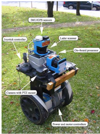
Fig. 1. The mapping robot: a Segway RMP equipped with scanning laser range finders (in both vertical and horizontal planes), a Garmin GPS unit and a MicroStrain IMU.
