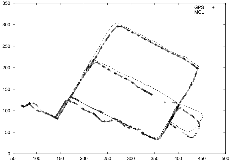
Fig. 4. Comparison of robot trajectory estimates using GPS and MCL; note that GPS estimates are sometimes unavailable due to satellite occlusion.
