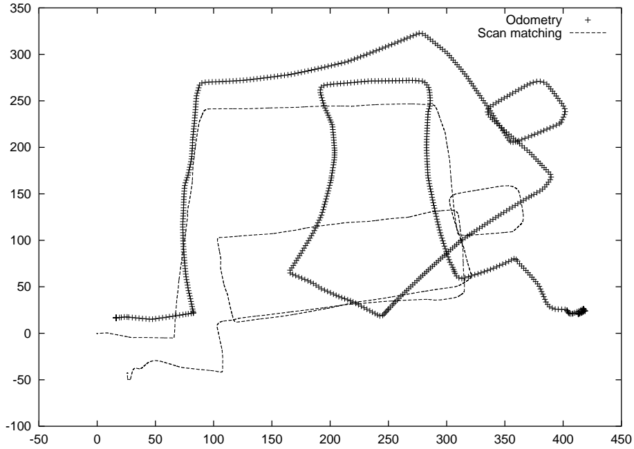
Fig. 3. Robot trajectory using odometry, and odometry plus laser scan matching. The robot executes a closed traverse of approximately 2 km.
