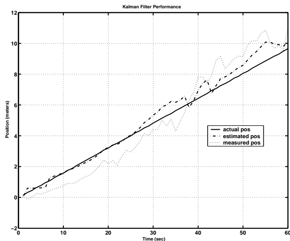
Figure 5: Kalman filter tracking performance
