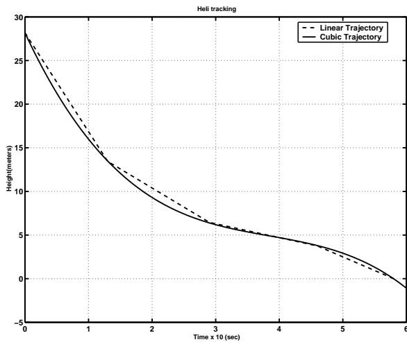
Figure 7: Height trajectory followed by the helicopter while tracking and landing
