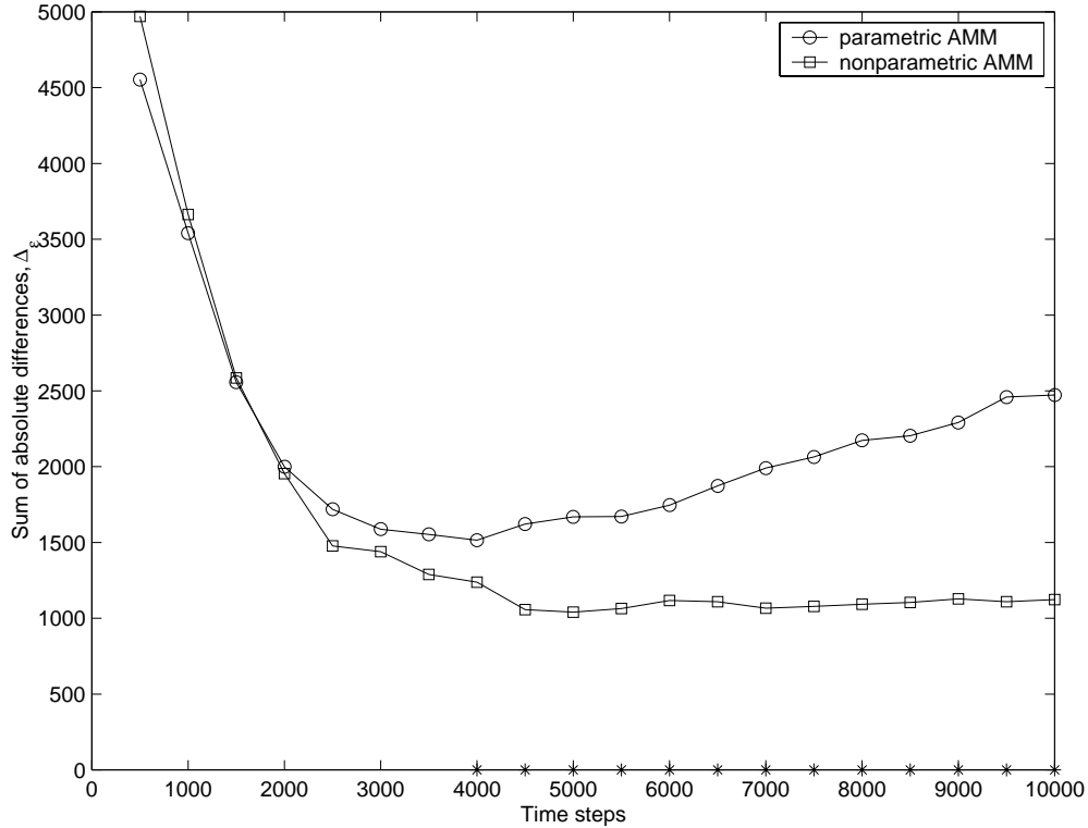
Figure 8.3: The performance, \Delta_\varepsilon , of parametric and nonparametric AMMs with a node-splitting significance of 0.05 and n_{\max} = 10 . This graph shows the average over 100 trials of 10000 simulation steps. Asterisks indicate a significant difference at a level of 0.01.
