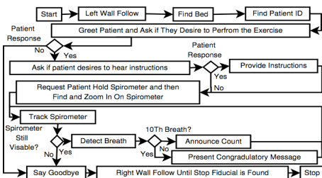
Control flow of Clara's architecture
