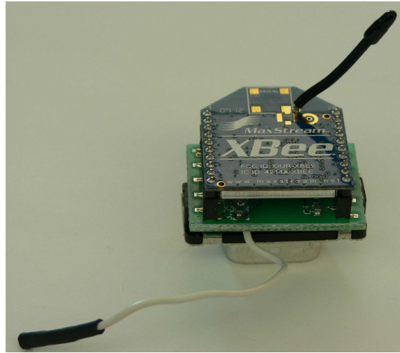
Fig. 27: XBee Wireless Communication Module.
