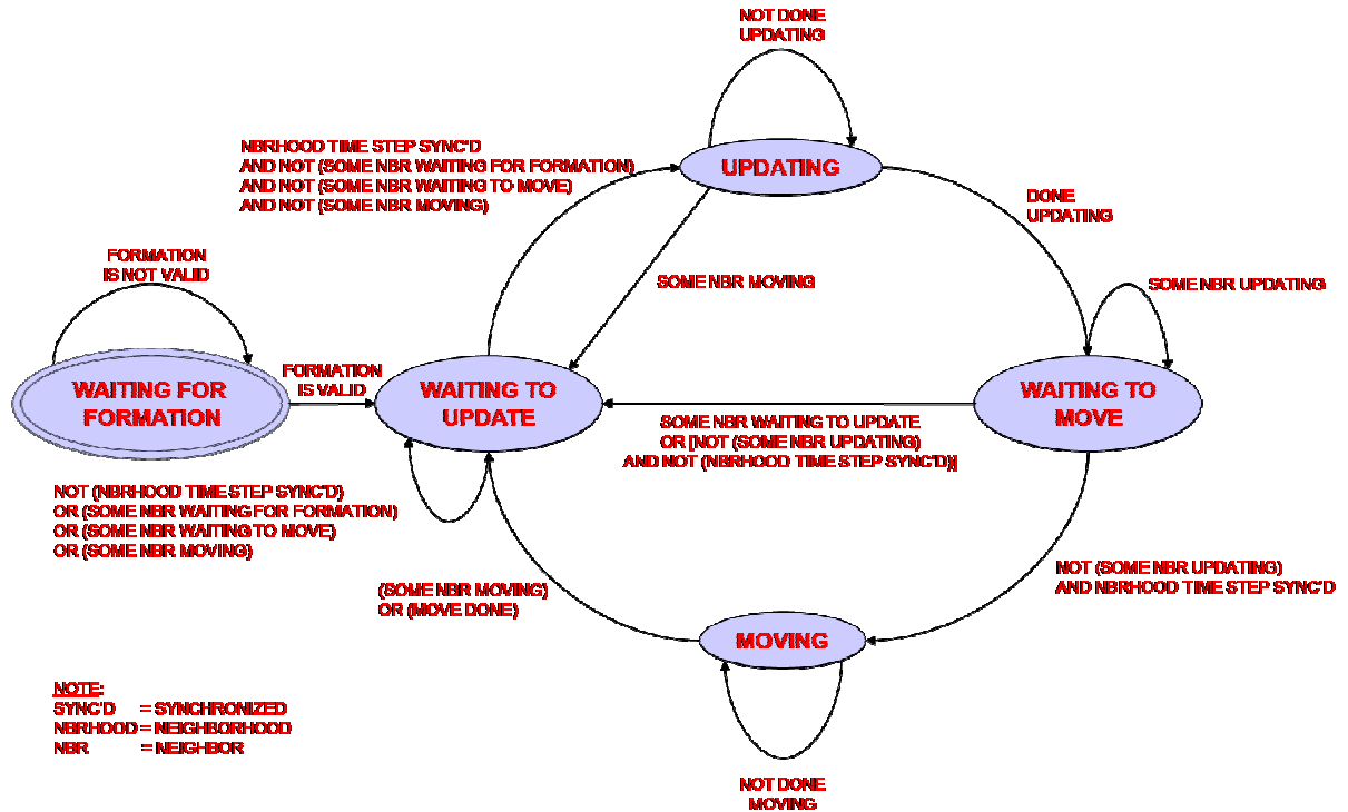
Fig. 28: Finite State Diagram of Robot Operation.
