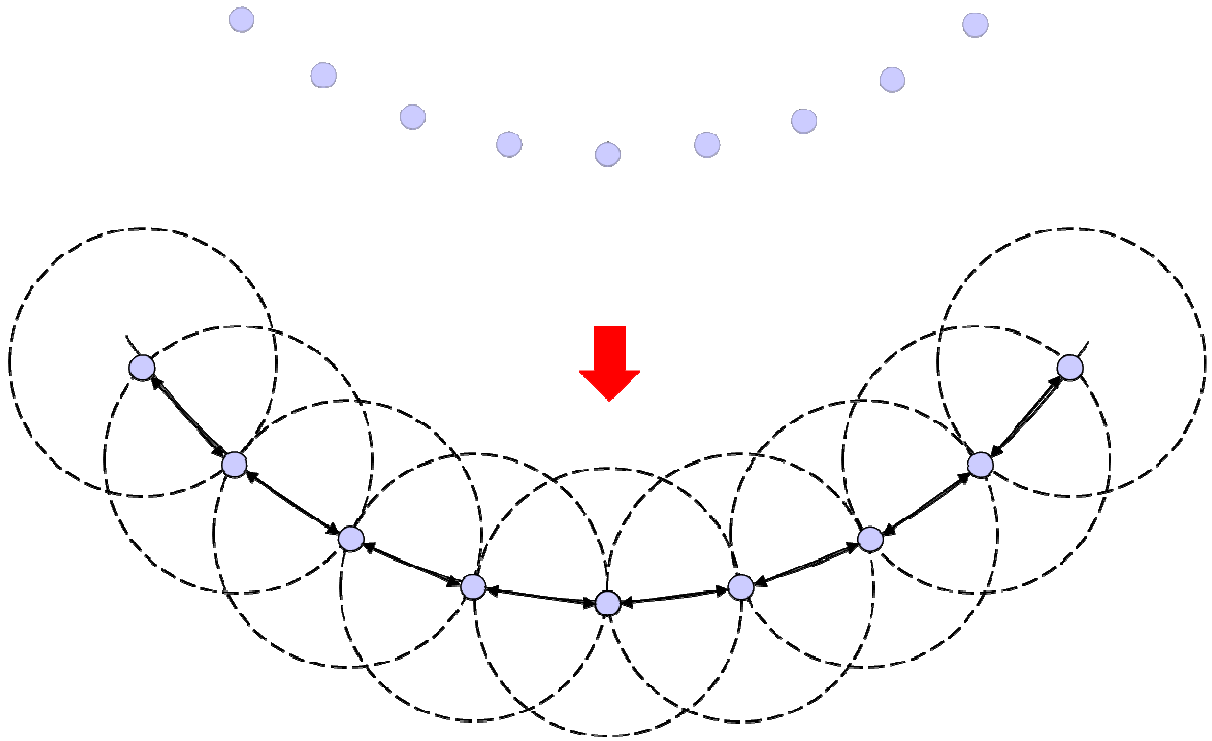
Fig. 21: Resizing Command Sent to a Seed Cell Changes Cell Interval in the Formation.
