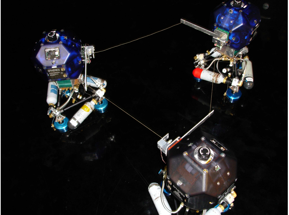
Fig. 9: Three SPHERES Satellites Maintain Formation by Keeping their Tethers Taut.
