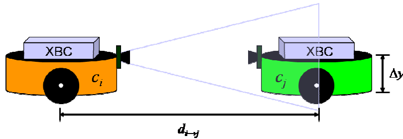
Fig. 26: c_i Identifies and Determines its Distance to c_j .
