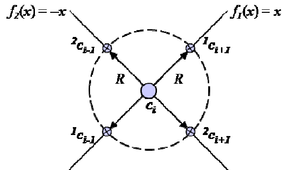
Fig. 33: A Formation Defined by Two Functions Yields Four Relationships.
