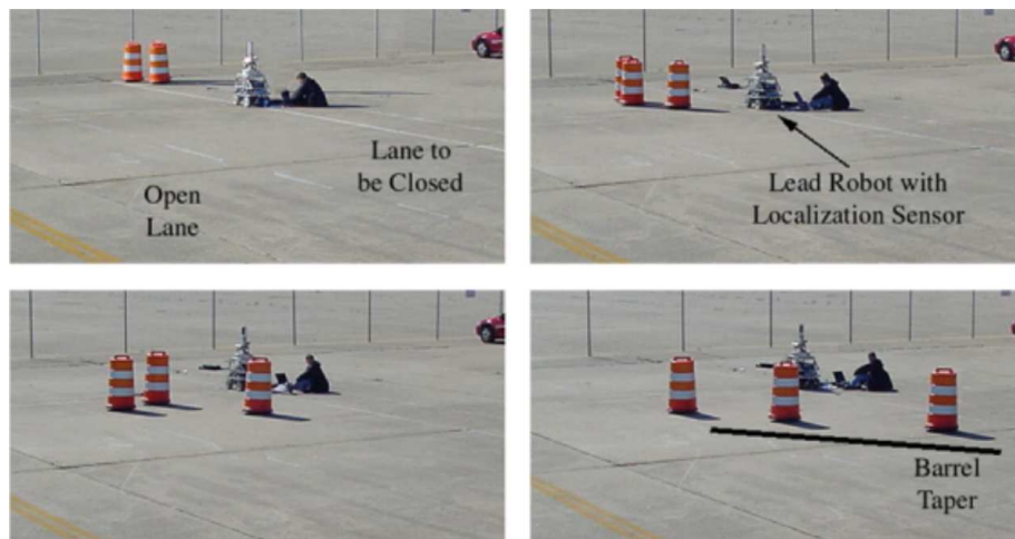
Fig. 3: Robotic Highway Safety Markers. [9]
