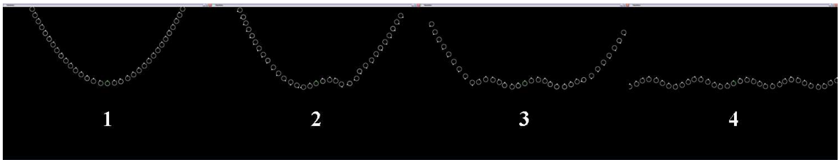
Fig. 23: Simulated Robots Change Formation from f(x) = x^2 (Parabola) to f(x) = 0.05 \sin(10 x) (Sine Curve); Pictured at Four Time Steps.
