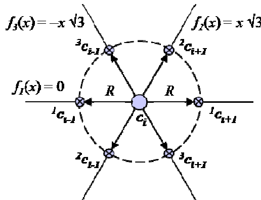
Fig. 30: A Formation Defined by Three Functions Yields Six Relationships.
