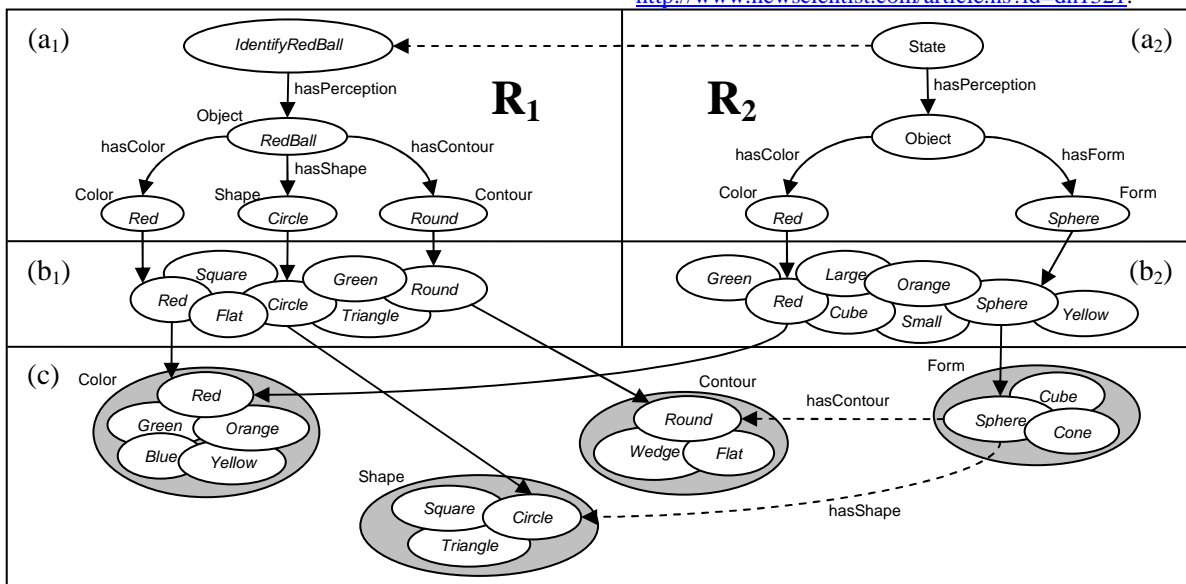
Figure 1: Solid lines denote explicit relationships; dotted lines denote inferred relationships. (a 1 ) symbolic definition of the goal state of a robot R_1 to identify a red ball; (a 2 ) the current perceptual state of the robot R_2 , which is inferred (by AIM) to be equivalent to the goal state of R_1 ; (b 1 & b 2 ) the known ontological concepts maintained and interpreted by AIM; (c) various concepts from the provided ontologies, shown with the necessary links to represent the goal.
