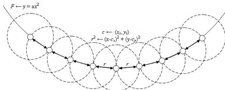
Figure 1: The cellular automata reactive control algorithm.
