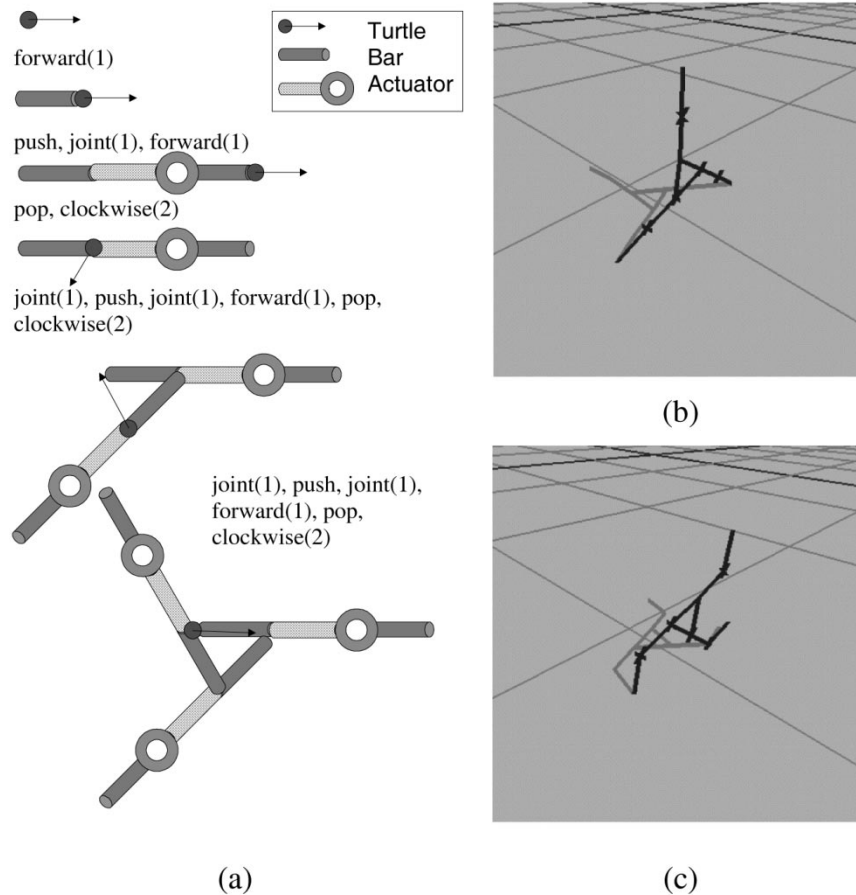
Fig. 3. Sample L-Robot. (a) Construction sequence leading to a tristar 2-D robot with three actuated joints. (b) Resulting robot, with joints at 180°. (c) With joints at 120°.
