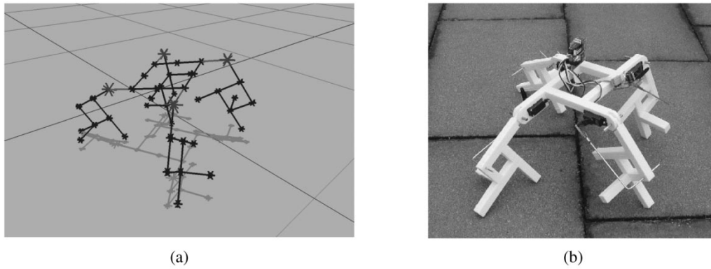
Fig. 8. An evolved 3D robot “Quatrobot”. (a) Simulated. (b) Physical. Notice the reuse of the leg assembly. For video of the robots in motion see http://www.demo.cs.brandeis.edu/pr/evo_design/evo_design/html .
