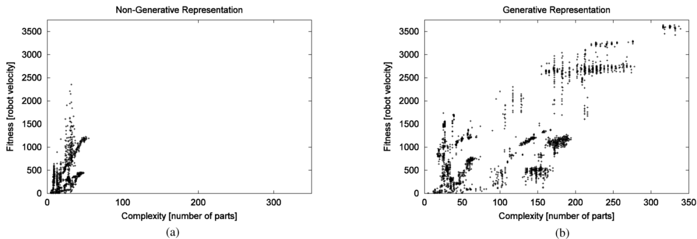
Fig. 10. Comparison of fitness versus number of parts. (a) Nongenerative representation. (b) Generative representation. One dot for the best individual of each generation for all 10 runs.
