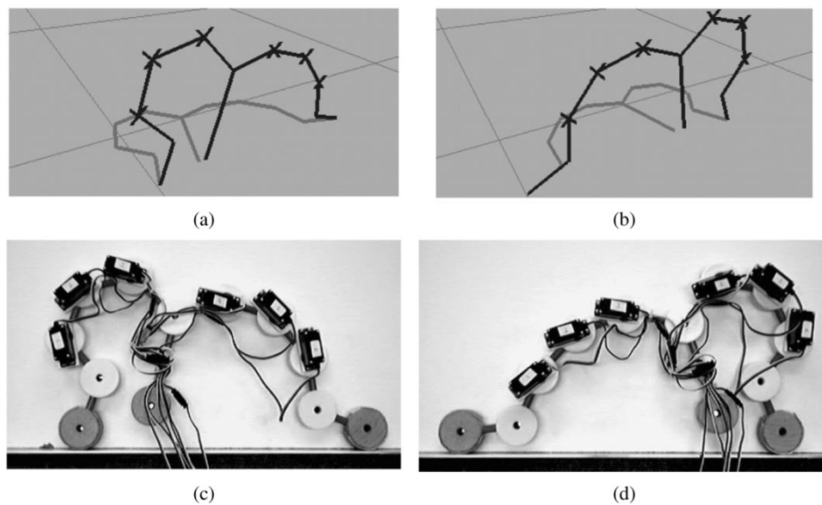
Fig. 6. Two parts of the locomotion cycle of an evolved 2-D robot “M”. (a, b) Simulated. (c, d) Physical. Notice regularity and symmetry.
