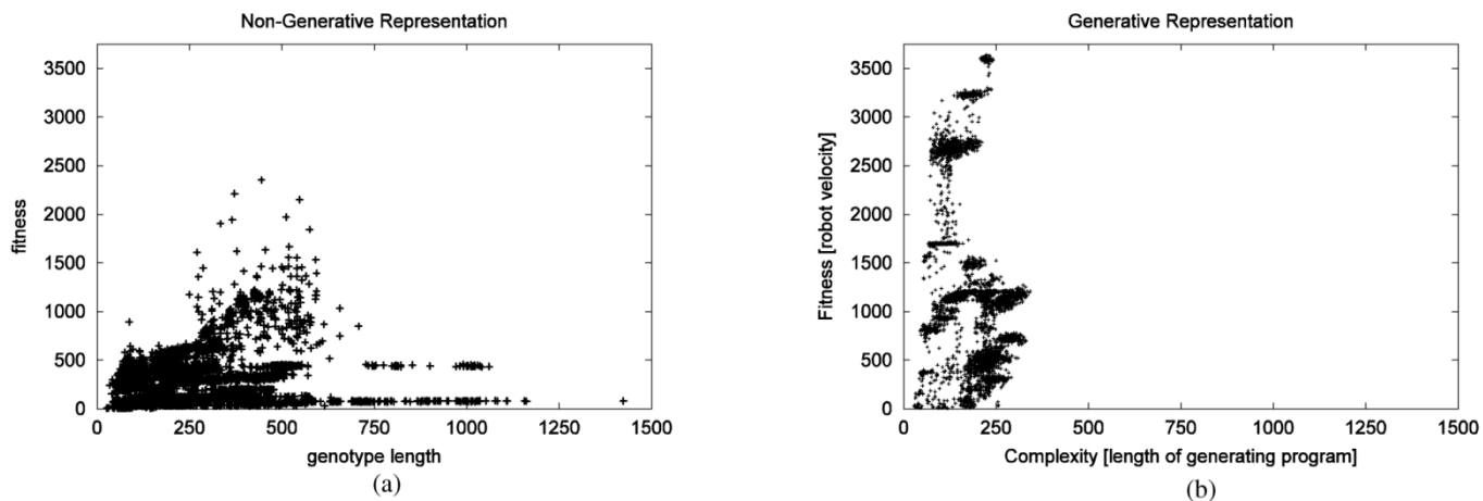
Fig. 11. Comparison of fitness versus length of generating program, measured in number of elements in encoded design. (a) Nongenerative representation. (b) Generative representation. One dot for the best individual of each generation for all ten runs.
