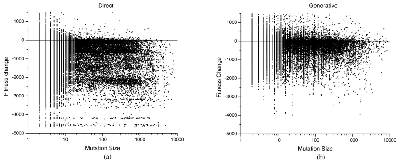
Fig. 12. Comparison of fitness change per mutation. (a) Nongenerative representation. (b) Generative representation.
