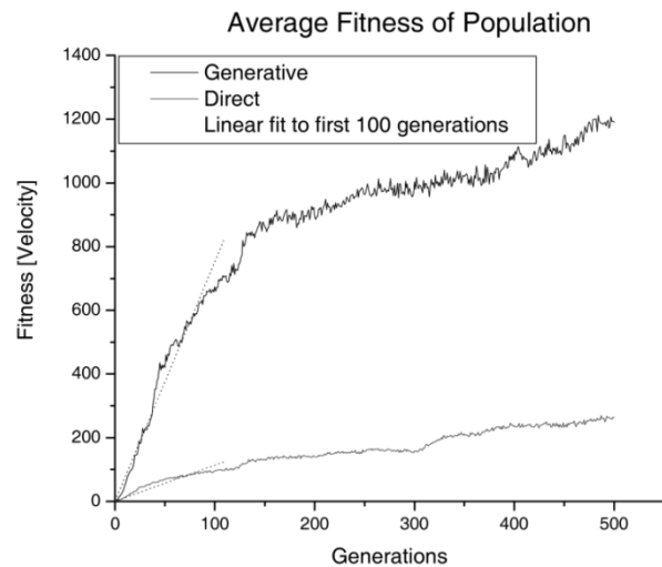
Fig. 9. Fitness over time, comparing nongenerative representation with generated representation. Data averaged over 10 runs.
