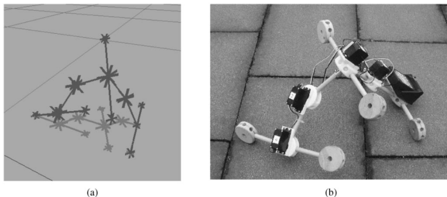
Fig. 7. An evolved 3D robot “Kayak”. (a) Simulated. (b) Physical. Notice the reuse of a T-junction.
