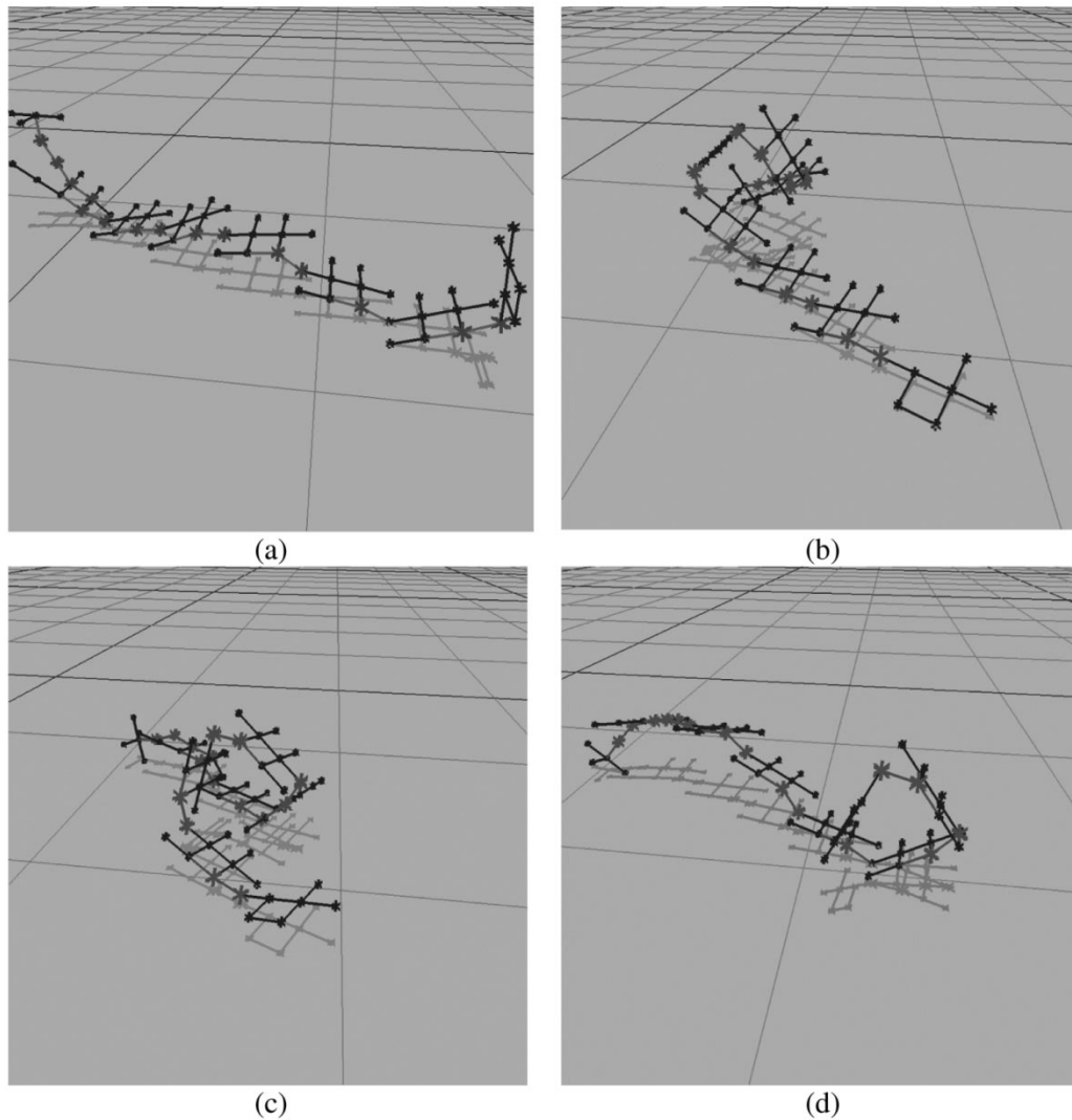
Fig. 5. The locomotion cycle of a 80-rod robot evolved using generative representation and reaching a fitness of 686. The robot moves by passing a loop from back to front. Frames (a–d) show four stages in the locomotion cycle. (For full motion, see video at http://www.demo.cs.brandeis.edu/pr/evo_design/evo_design.html ).
