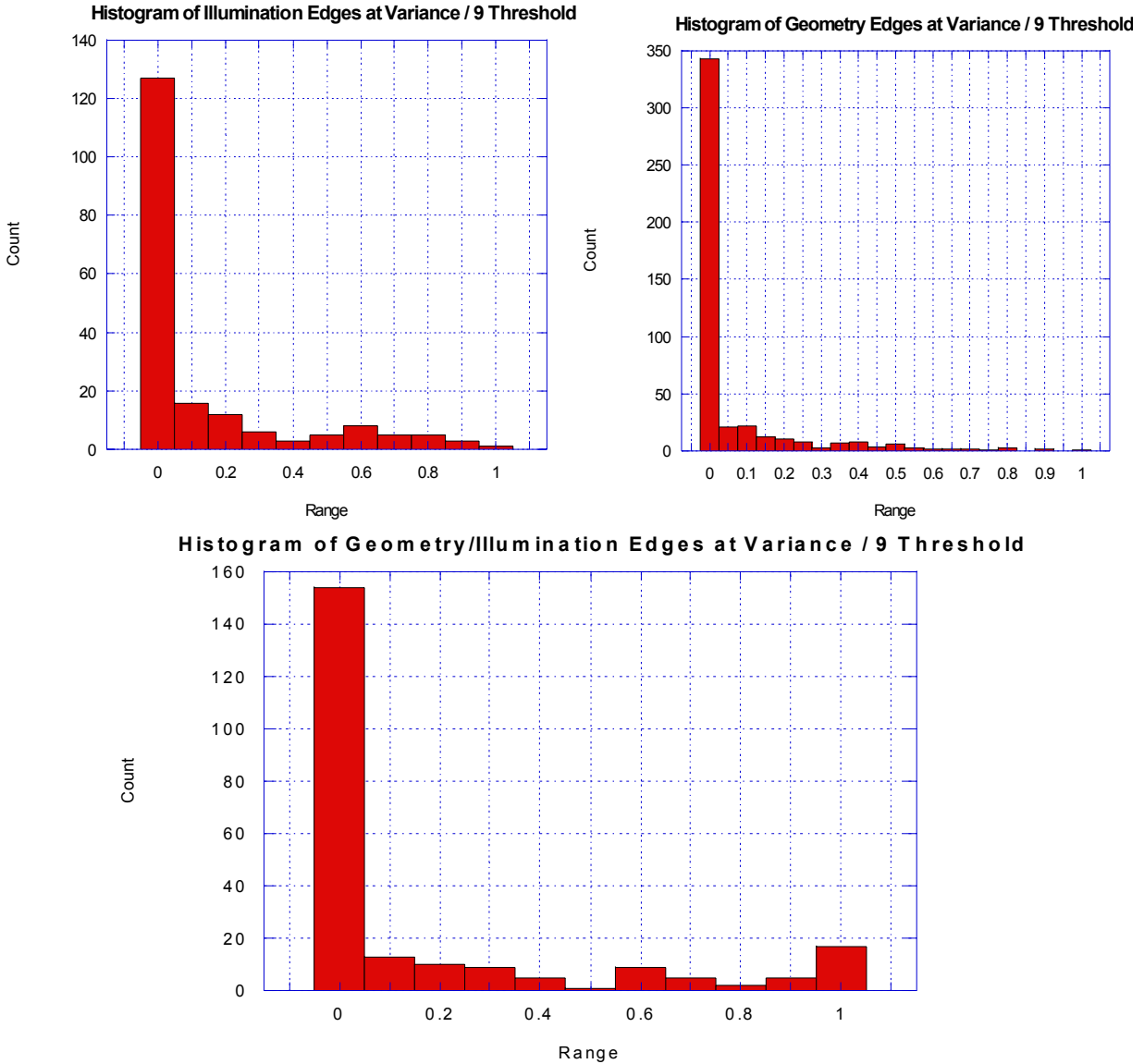
Figures 4, 5, and 6: Histograms of model fitting for non-material edges
