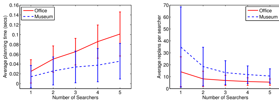
Figure 3.11: Average planning time for FHPE+SA with synchronous sequential planning (left). Error bars are one standard deviation. The planning time scales linearly with the team size. Average replans required per searcher to find a randomly moving target (right). Even with the highest number of replans, the total planning time is less than two seconds.
