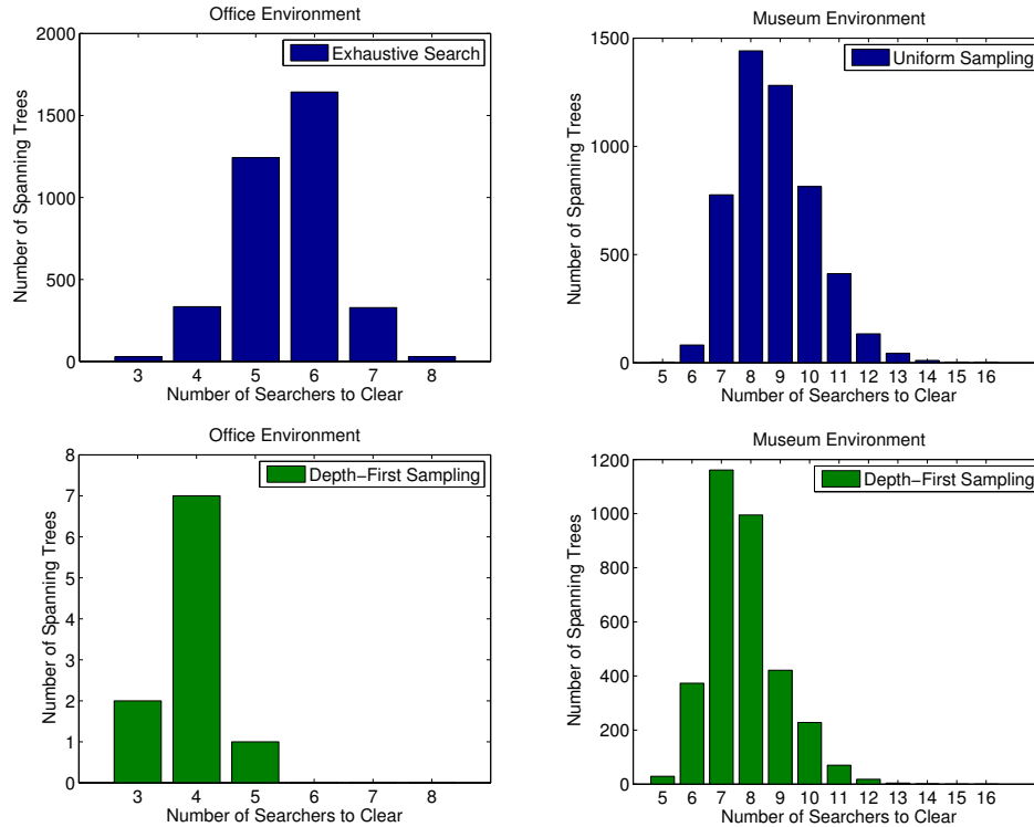
Figure 4.5: Histograms of number of searchers to clear the office (left) and museum (right) using labeled traversal on many different spanning trees. In the office, exhaustive search is compared to depth-first sampling. Depth-first sampling limits the space of spanning trees searched but generates trees that require fewer searches. In the museum, uniform sampling of 30,000 trees is substituted for exhaustive search. Again, depth-first sampling generates spanning trees requiring fewer searchers.
