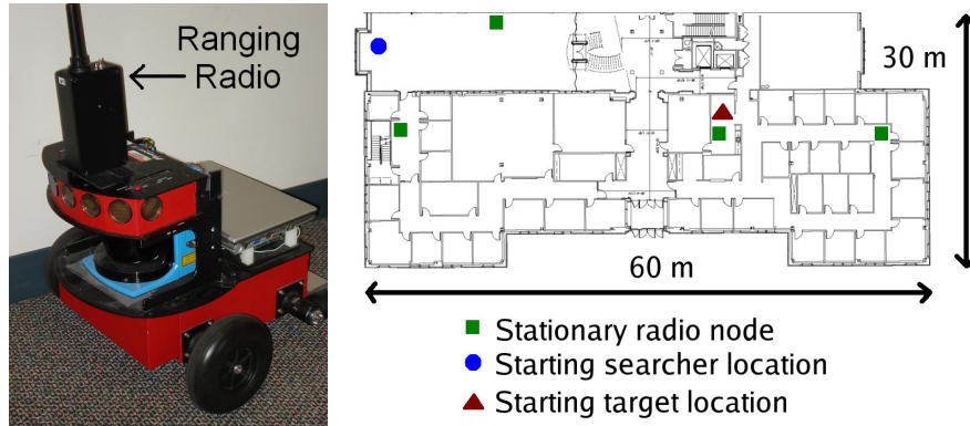
Figure 3.7: Photograph of Multispectral ultra-wideband ranging radio mounted on Pioneer robot (left) and floorplan of testing environment (right). The robot was teleoperated around the environment to act as the moving target.
