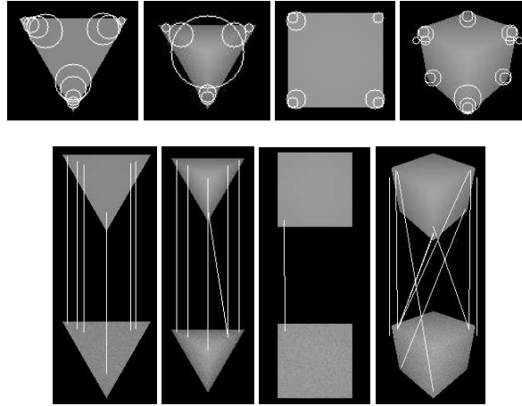
Fig. 3 Top: SURF features extracted from viewing depth maps of tetrahedron and cube faces and vertices. Bottom: SURF feature correlations when compared to noisy depth maps.
