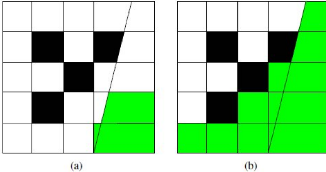
Fig. 3. The neighborhood that can be moved to, M_1 (a) and the neighborhood that can be seen, N_1 (b), from area F_1 .
