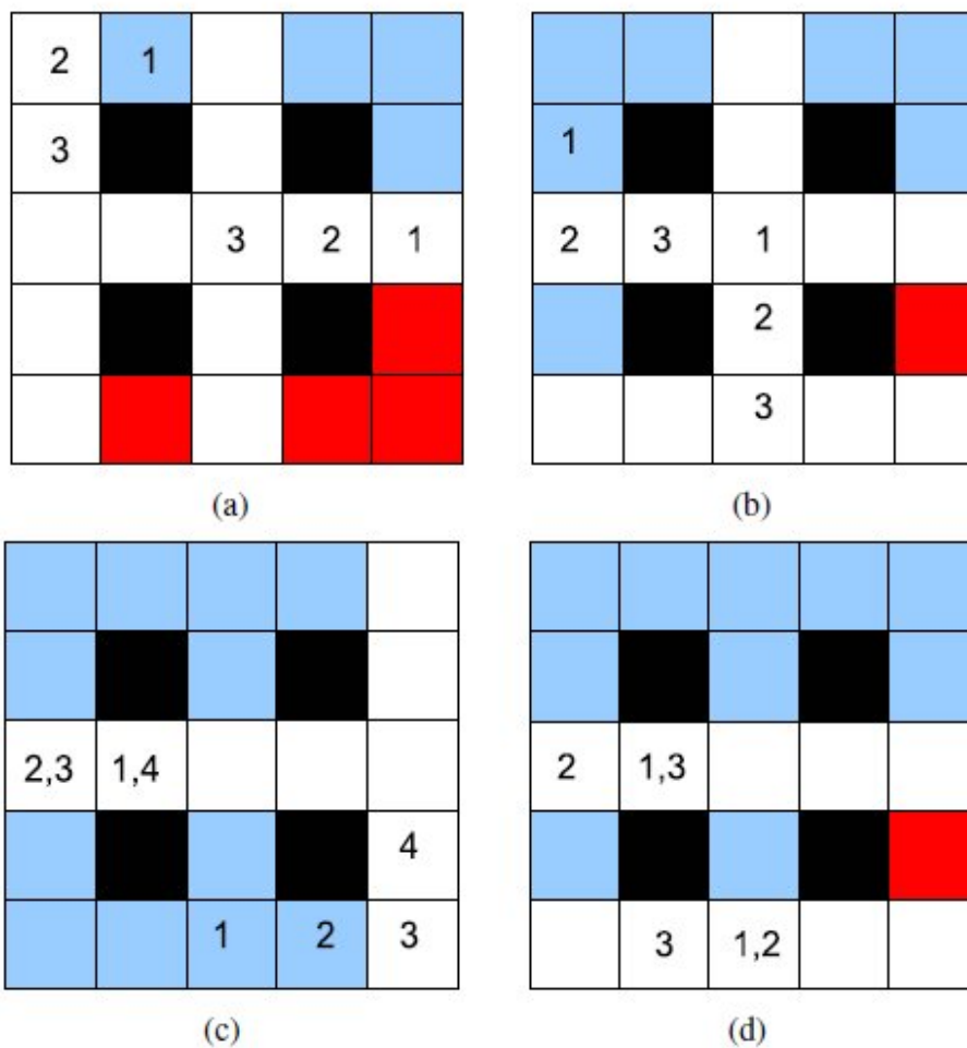
Fig. 6. The results of running the algorithm on a manhattan grid with four obstacles. The partition is shown in Figure 5, and the search problem is solved with 2 pursuers in three iterations where the results of iteration 1, 2 and 3 are shown in (a), (b) and (c) respectively. Note that 4 time steps were necessary in iteration 3, the result of the third iteration with 3 time steps is showed in (d). White regions are in state S_1 and S_2 , blue regions are in state S_3 , whereas red regions are in state S_4 .
